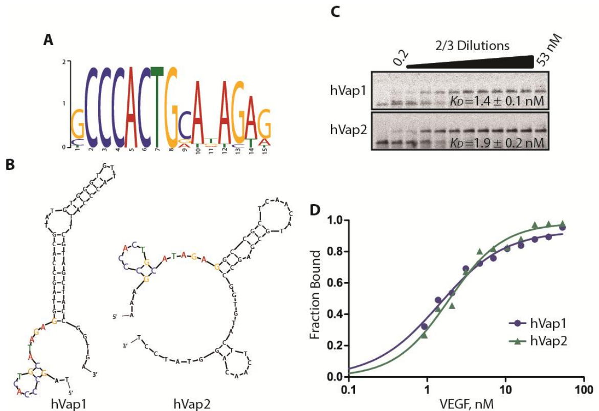
Figure 3-3. Determining consensus motif, secondary structure, and solution affinity of the aptamers against VEGF. (a) The consensus motif shared among the top ten highly enriched sequences against VEGF was identified using the MEME Suite ( http://meme.nbcr.net/meme/ ). (b) Shown are the secondary structures of the 60-nt variable region of the top two aptamers, hVap1 and hVap2, predicted by Mfold ( http://mfold.rna.albany.edu/ ). (c-d) Solution affinity ( K_D ) of the full-length hVap1 and hVap2 against VEGF was determined by F-EMSA (c), and by fitting the Hill equation to the data (d). VEGF was used at a series of 2/3-fold serial dilutions starting at 53 nM, while labeled aptamers were used at 500 pM.
