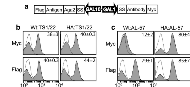
FIGURE 4. Detection of specific interactions between antibodies and antigens in YS2H. a , schematic diagram of the expression cassette used to study antigen (bait) and antibody (prey) interactions. b and c , shown are the histograms of the interactions of the wild-type and the high affinity (HA) I domains as baits and activation-insensitive antibody, TS1/22 ( b ) activation-specific antibody, AL-57 ( c ) as preys. Filled histograms are of antibody binding to Myc and FLAG tags to the induced clones. Thin black lines represent antibody binding to uninduced clones as controls. The numbers in each plot indicate the means \pm S.E. of the MFI of the filled histograms from three independent measurements.
